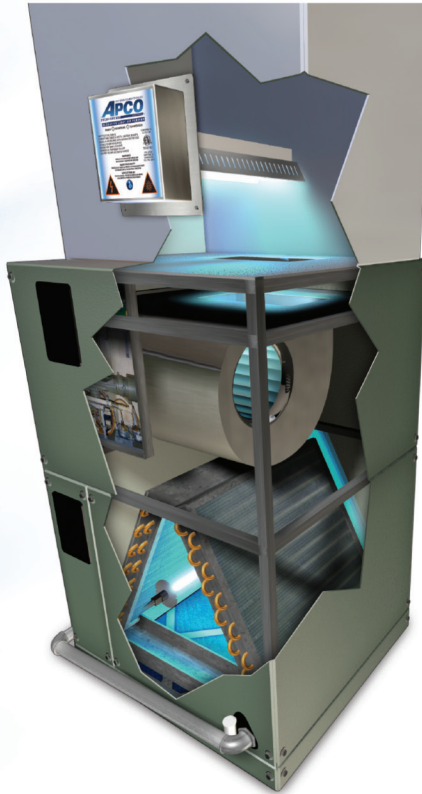
APCO ® Dual Installed in Air Handler
